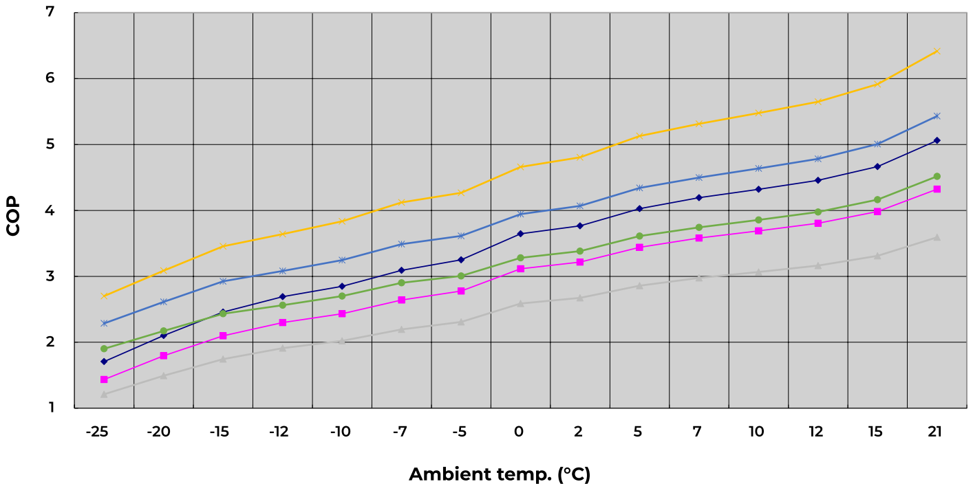
Curve of COP Performance
