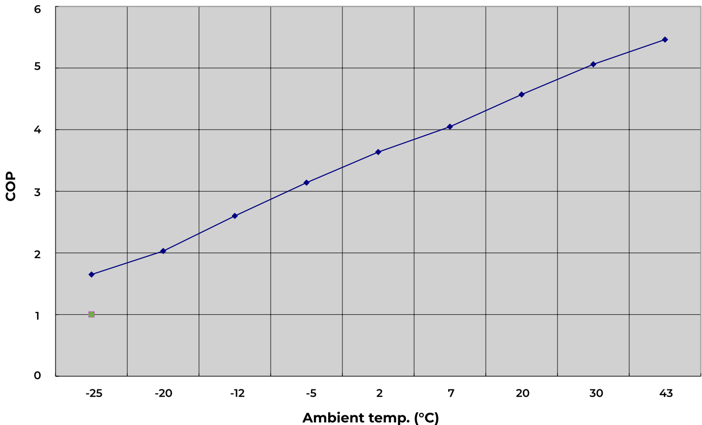
Curve of COP Performance
